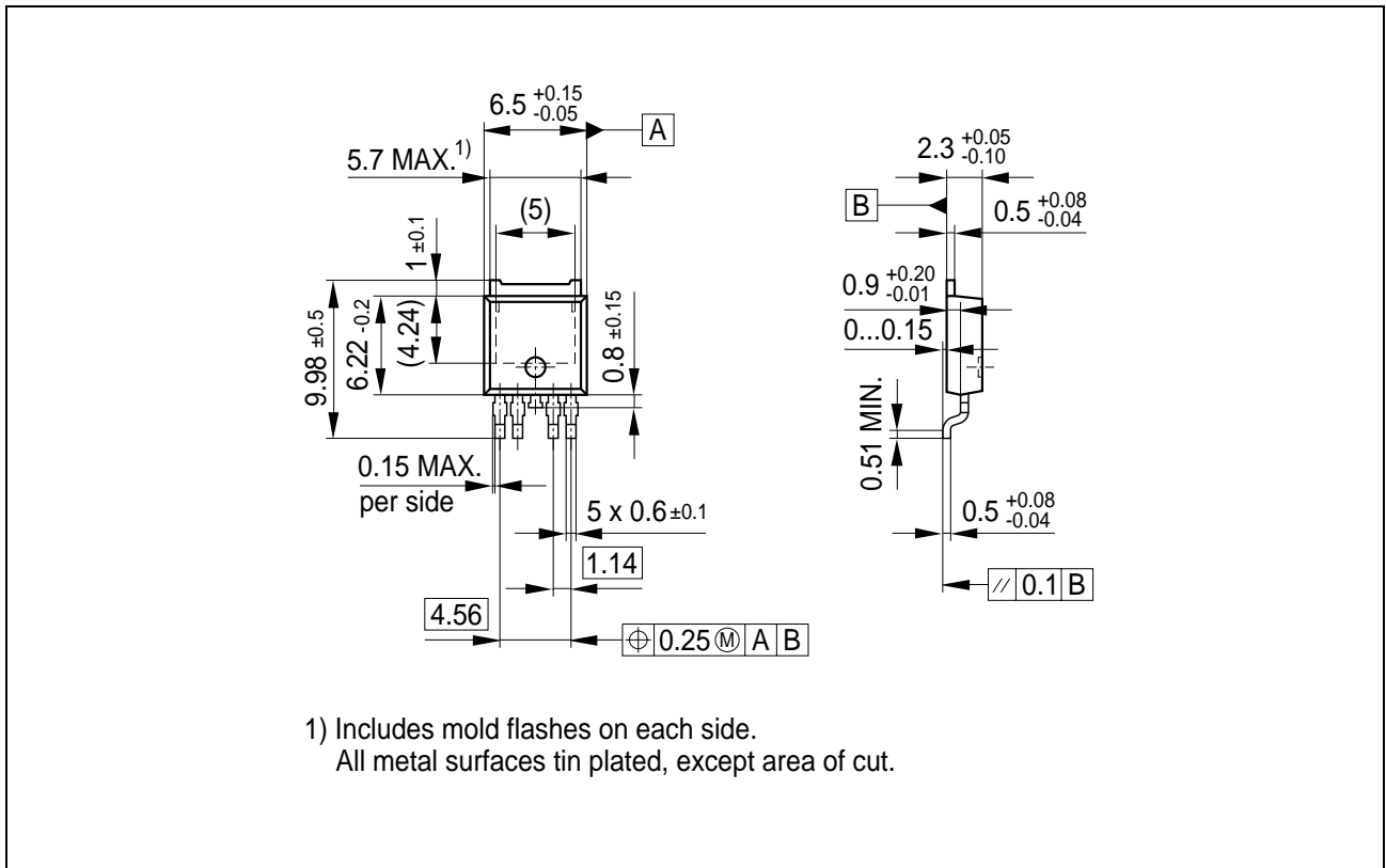
Figure 5 P-TO252-5-11 (Plastic Transistor Single Outline)
